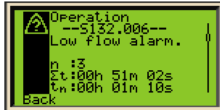
Diagnostics Display
